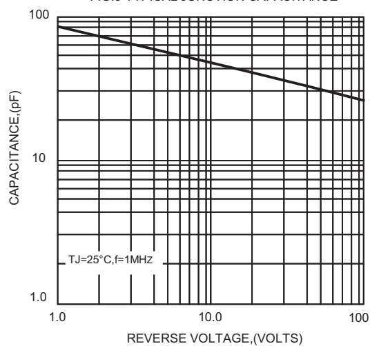
FIG.3-TYPICAL JUNCTION CAPACITANCE
