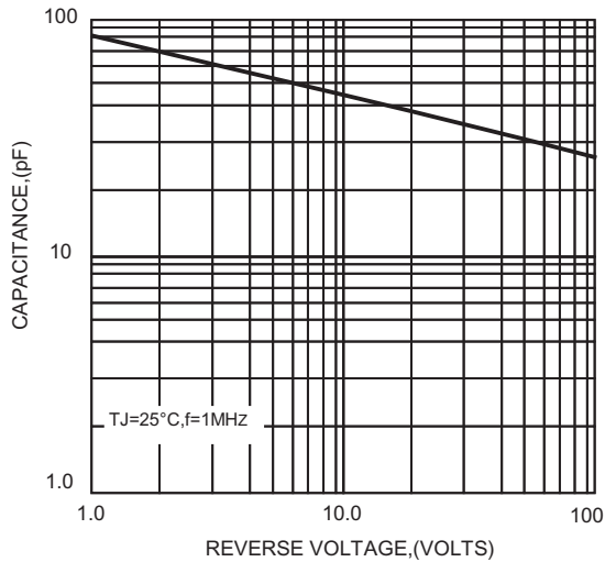
FIG.3-TYPICAL JUNCTION CAPACITANCE
