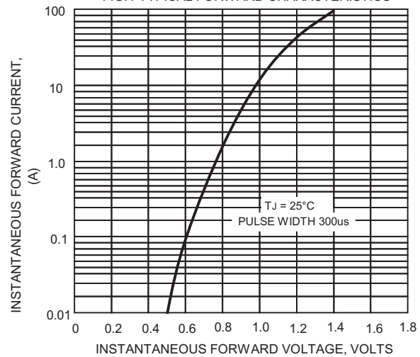
FIG.4-TYPICAL FORWARD CHARACTERISTICS
