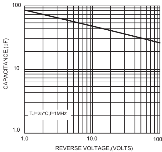
FIG.3-TYPICAL JUNCTION CAPACITANCE
