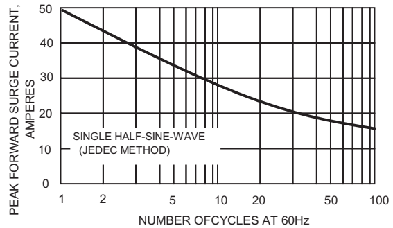
FIG.2-MXIMUM NON-REPETITIVE SURGE CURRENT
