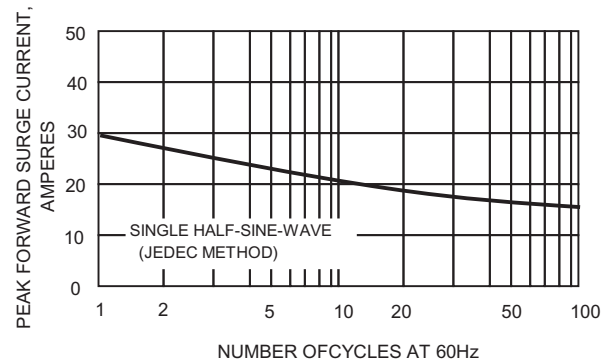
FIG.2-MXIMUM NON-REPETITIVE SURGE CURRENT
