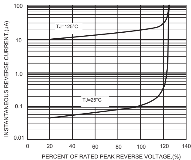
FIG.5-TYPICAL REVERSE CHARACTERISTICS
