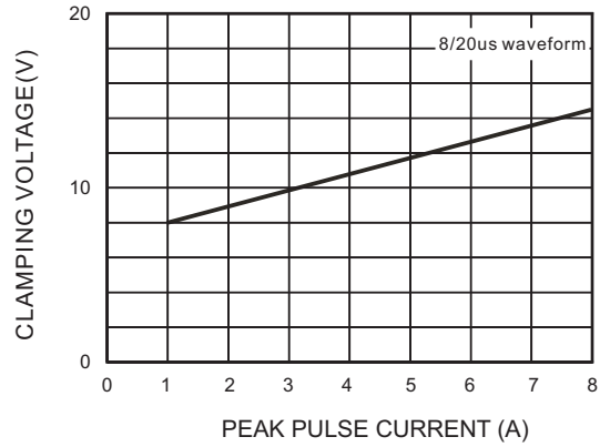
FIG.2- TYPICAL CLAMPING VOLTAGE VS. PEAK PULSE CURRENT
